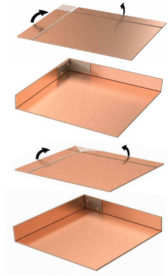
Examples for the rivet arrangement as a function of the corner cut for peripheral bent edge formats
