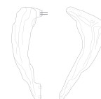
EA1029 Door Hardware - Door Pull H 260 mm | 10,24" L 130 mm | 5,12" D 65 mm | 2,56"
