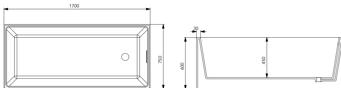
Vasca Venus Venus Bathtub Cod. VAVE
