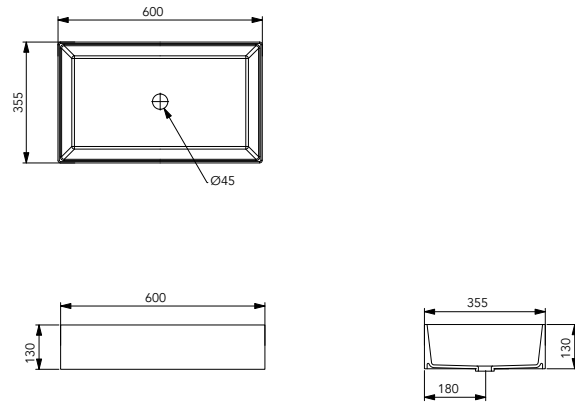
cod. BXLA60 Bacino in crystal-tech® cm60 Float in crystal-tech® cm60
