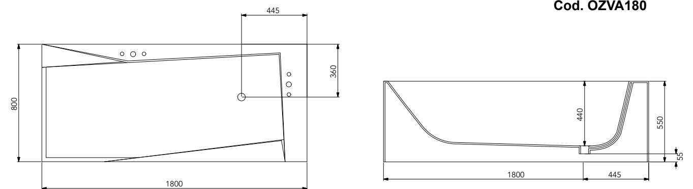
Vasca Oz Oz Bathtub Cod. OZVA180
