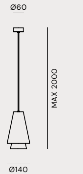
281.03.ON LED 5W 2700K
