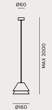
281.01.ON LED 5W 2700K
