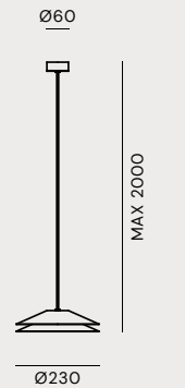
281.02.ON LED 5W 2700K
