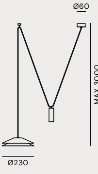
281.05.ON LED 5W 2700K
