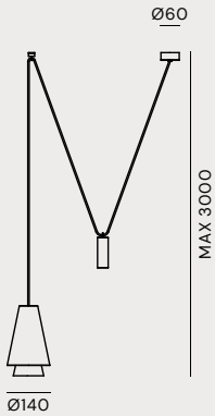
281.06.ON LED 5W 2700K
